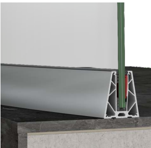
M8208 on-floor and curved, with 8+8mm and 10+10mm glass
